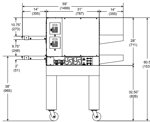
SIDE VIEW (ONE MODULE WITH BASE)
